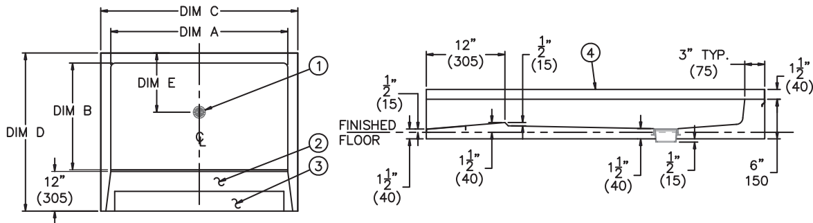
TERRAZZO-WARE SHOWER BASES WITH ADA RAMP
