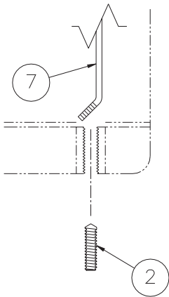
SPRAYHEAD SECTION INSTALLATION DETAIL
