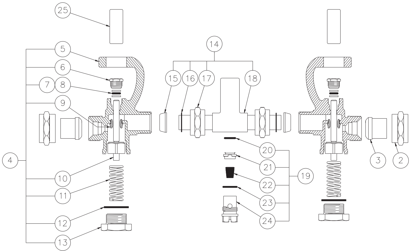
1 COMPLETE ASSY
