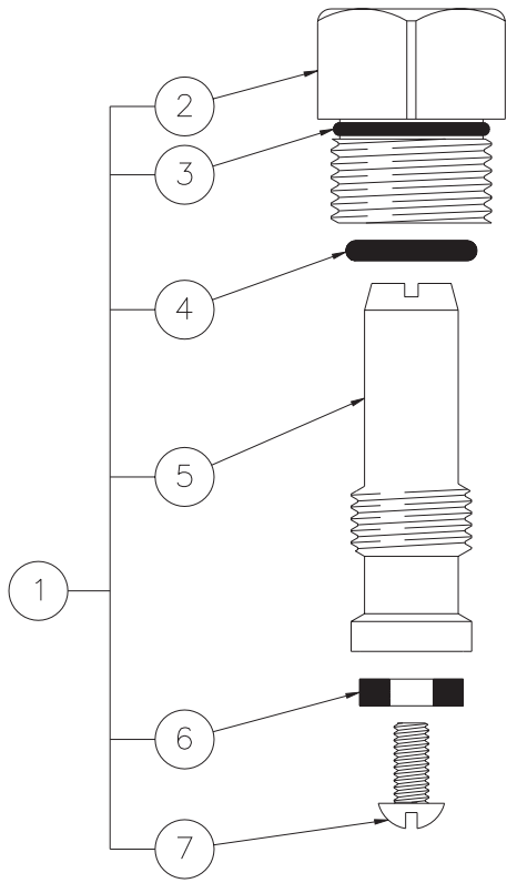
STOP ASSEMBLY
