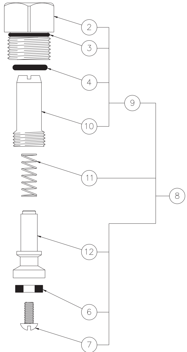
CHECKSTOP ASSEMBLY
