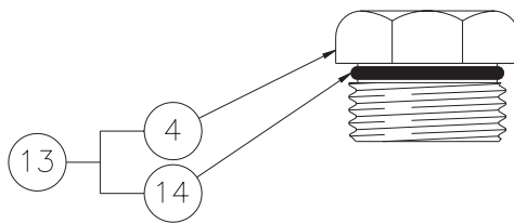
'NO STOP' PLUG ASSEMBLY
