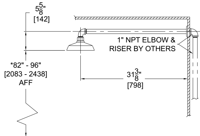
S2200-RA
