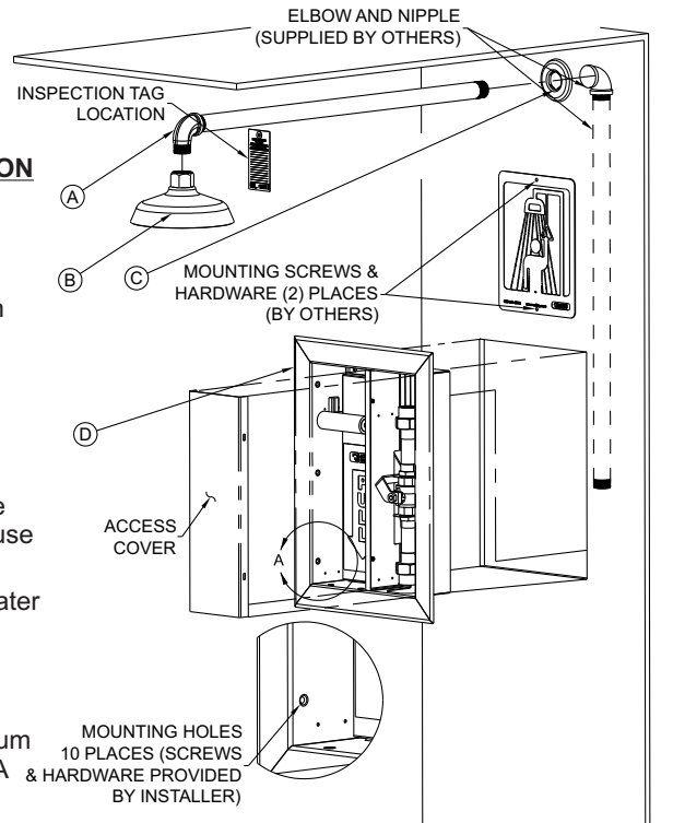
S2200-RA
