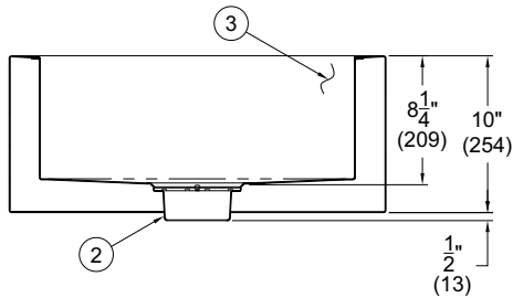
SECTION VIEW A-A
