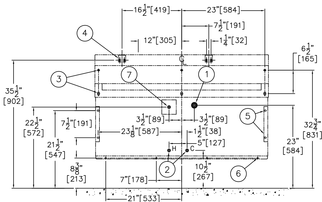
FRONT VIEW
