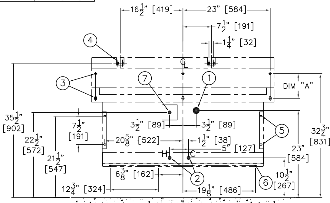
FRONT VIEW
